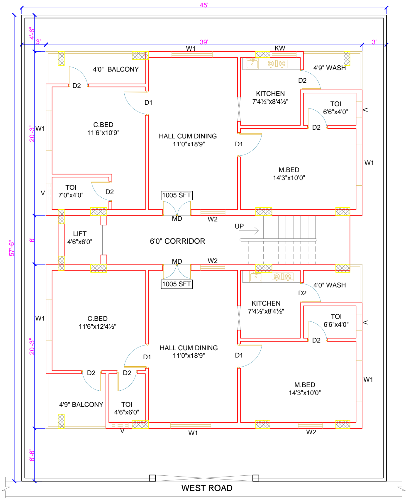
TYPICAL FLOOR PLAN WITH SET BACK DEVIATION
